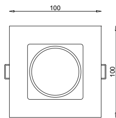
LI102x
